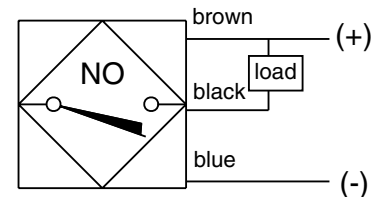
BTPX-N (NPN) (Current sinking)
