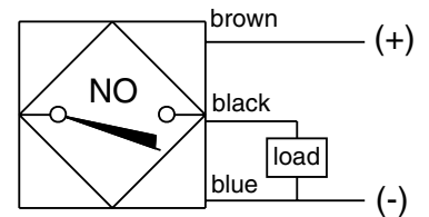
BTPX-P (PNP) (Current sourcing)
